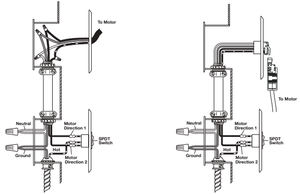
Standard Hard wiring
